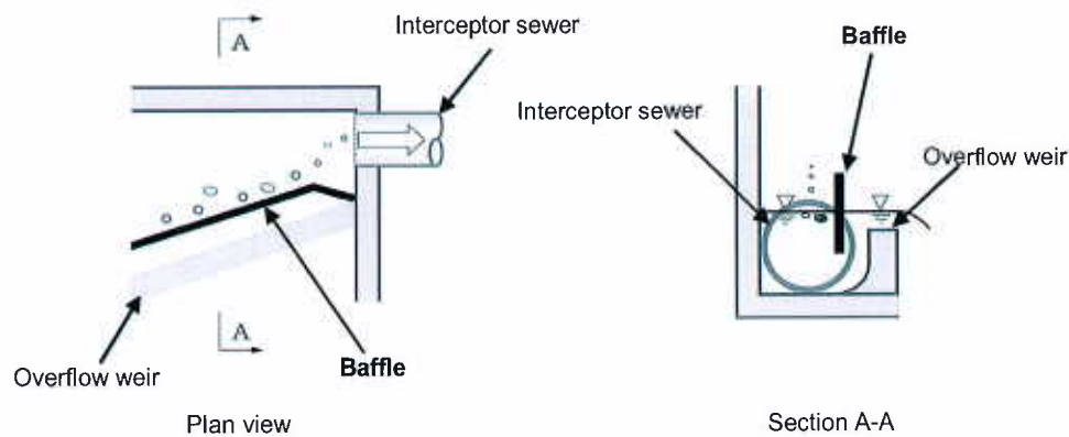
Fig.2 Baffle
